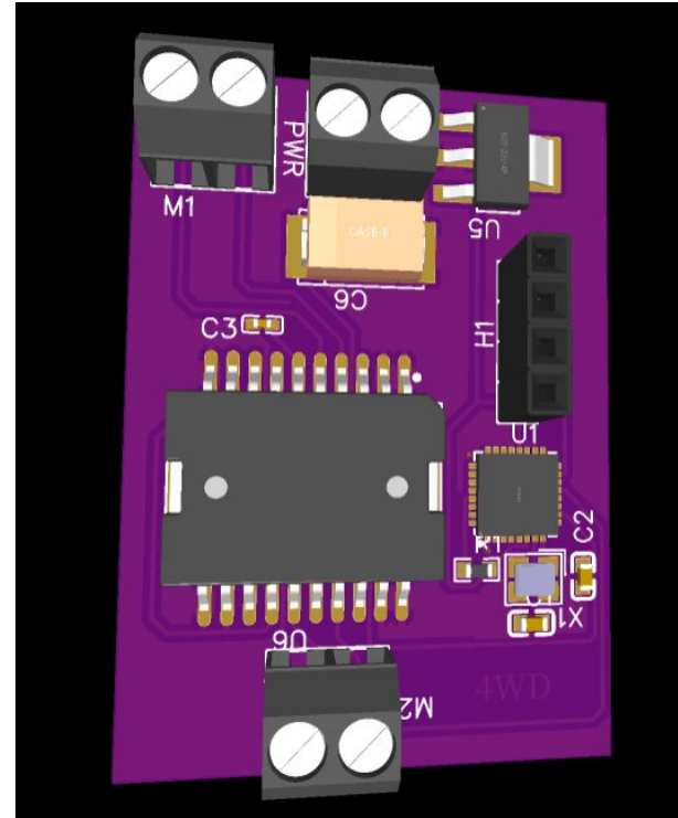
PCB of Receiver and control unit
