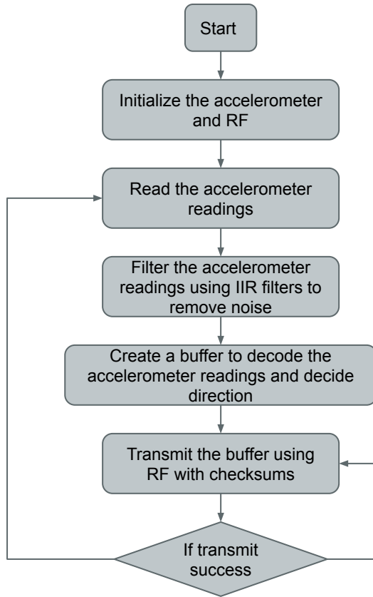
Flowchart of the Transmitter and Sensor unit
